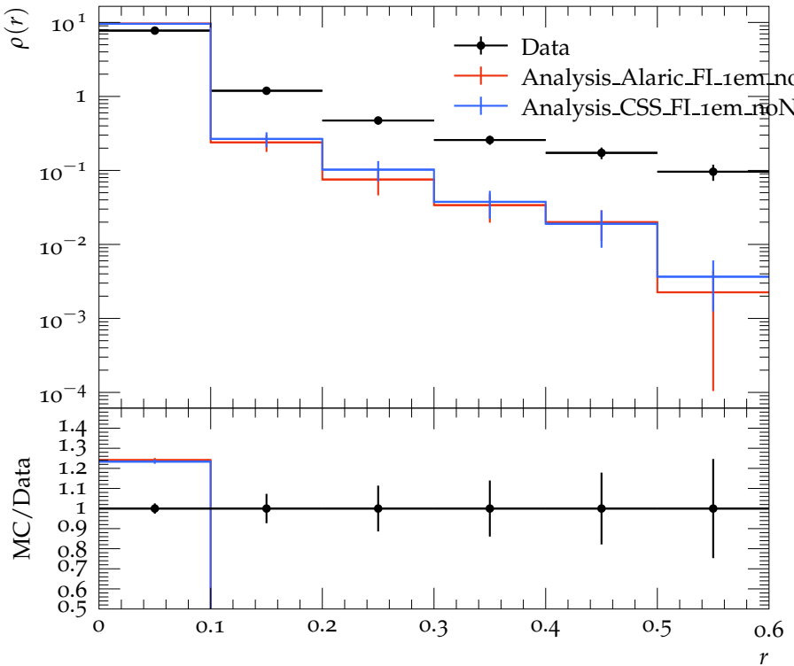
Jet shape \rho for p_{\perp} \in 260\text{--}310 GeV, y \in 2.1\text{--}2.8
