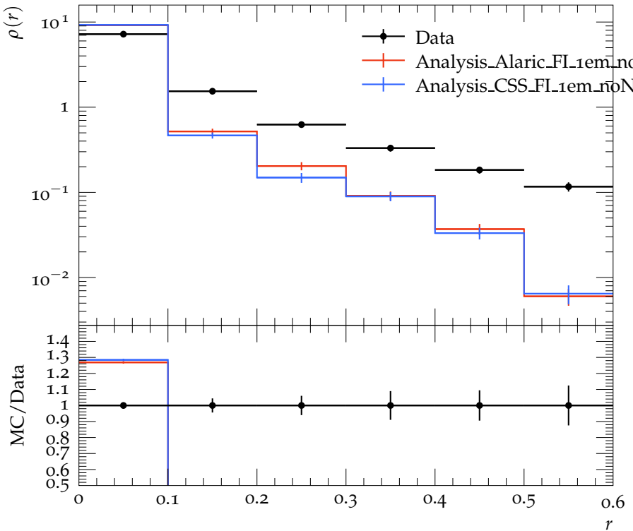
Jet shape \rho for p_{\perp} \in 260\text{--}310 GeV, y \in 0.3\text{--}0.8
