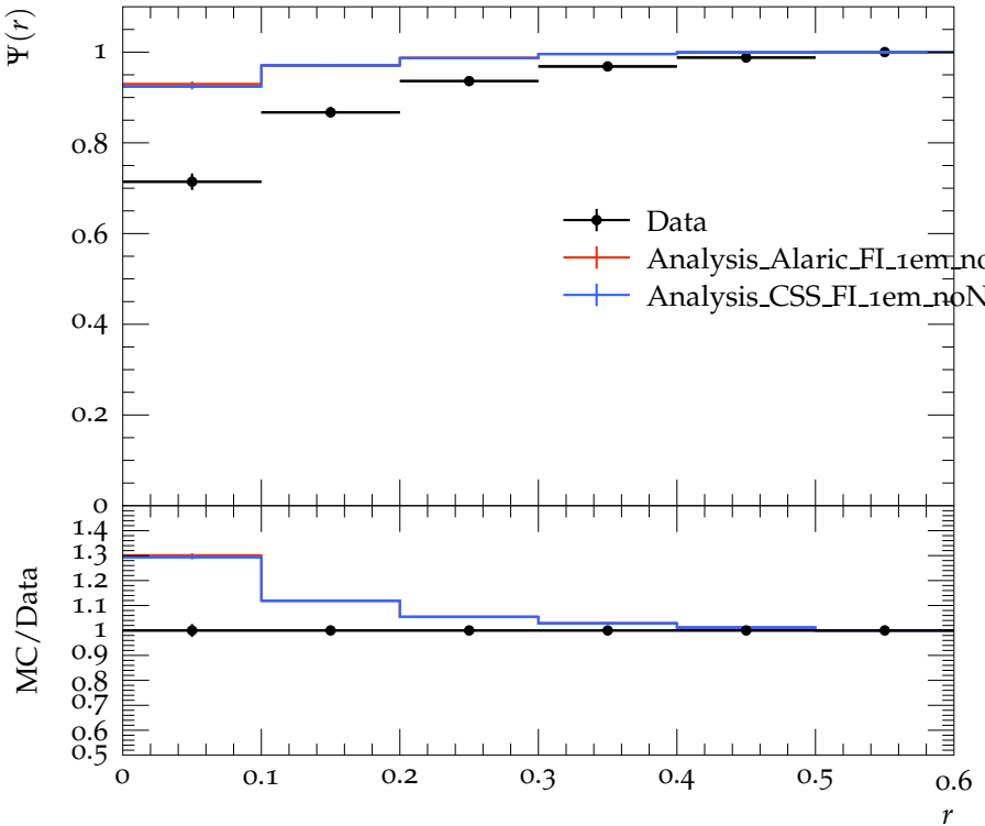
Jet shape \Psi for p_{\perp} \in 260\text{--}310\text{ GeV} , y \in 0.0\text{--}0.3
