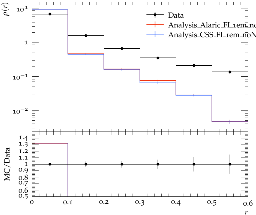
Jet shape \rho for p_{\perp} \in 210\text{--}260 GeV, y \in 0.0\text{--}2.8
