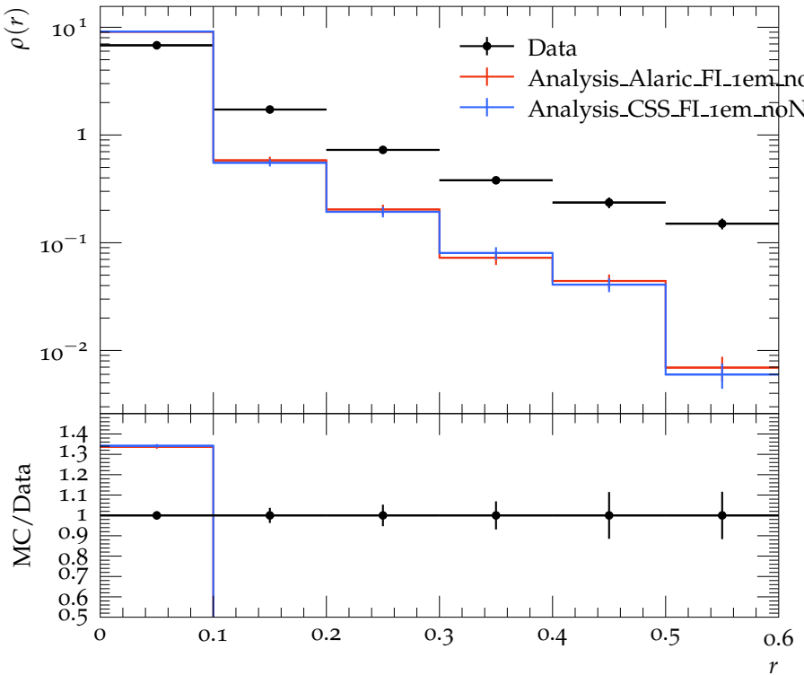
Jet shape \rho for p_{\perp} \in 210\text{--}260 GeV, y \in 0.0\text{--}0.3
