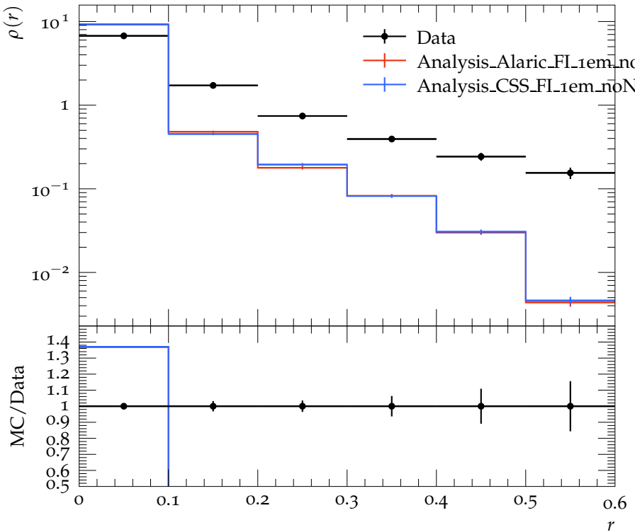
Jet shape \rho for p_{\perp} \in 160\text{--}210\text{ GeV} , y \in 0.0\text{--}2.8
