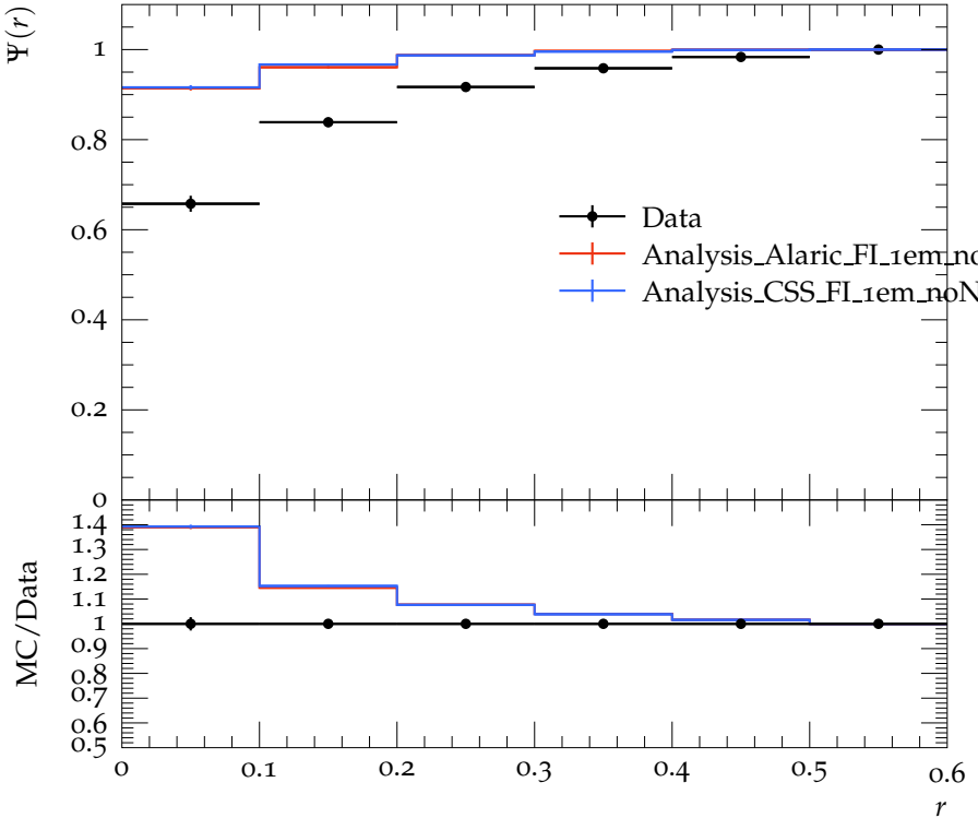
Jet shape \Psi for p_{\perp} \in 160\text{--}210\text{ GeV} , y \in 0.0\text{--}0.3
