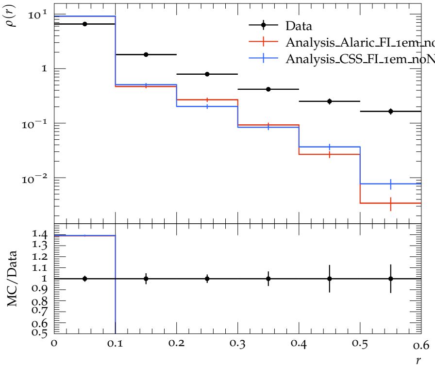
Jet shape \rho for p_{\perp} \in 160\text{--}210\text{ GeV} , y \in 0.0\text{--}0.3
