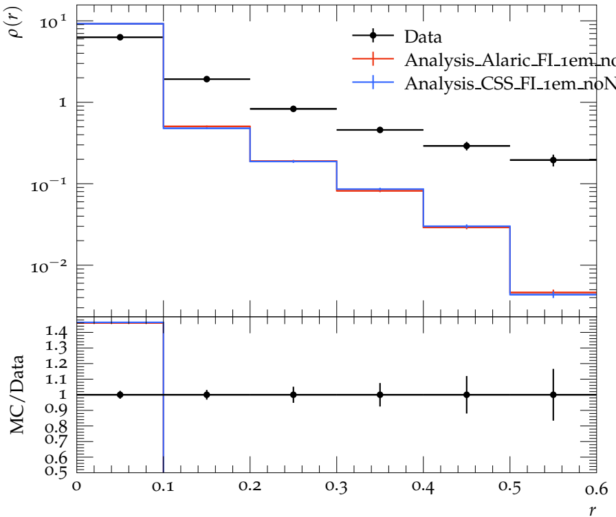
Jet shape \rho for p_{\perp} \in 110\text{--}160\text{ GeV} , y \in 0.0\text{--}2.8
