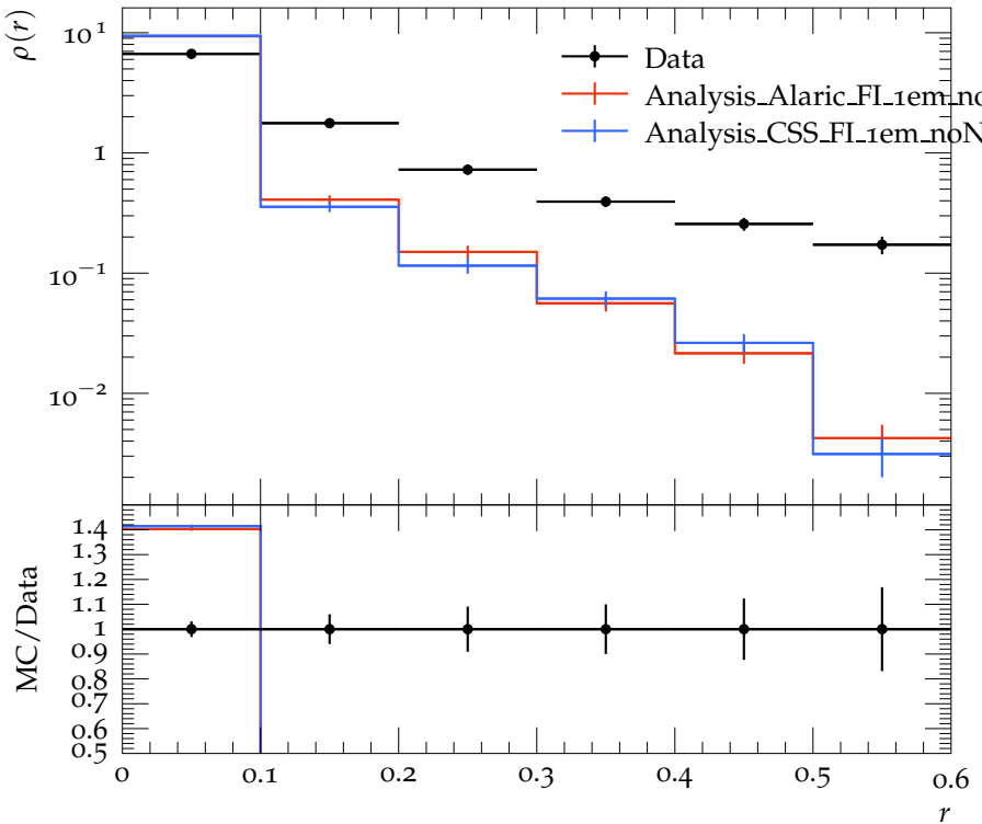
Jet shape \rho for p_{\perp} \in 110\text{--}160\text{ GeV} , y \in 2.1\text{--}2.8
