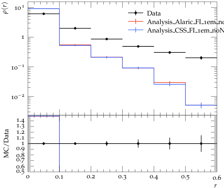
Jet shape \rho for p_{\perp} \in 110\text{--}160\text{ GeV} , y \in 0.0\text{--}0.3
