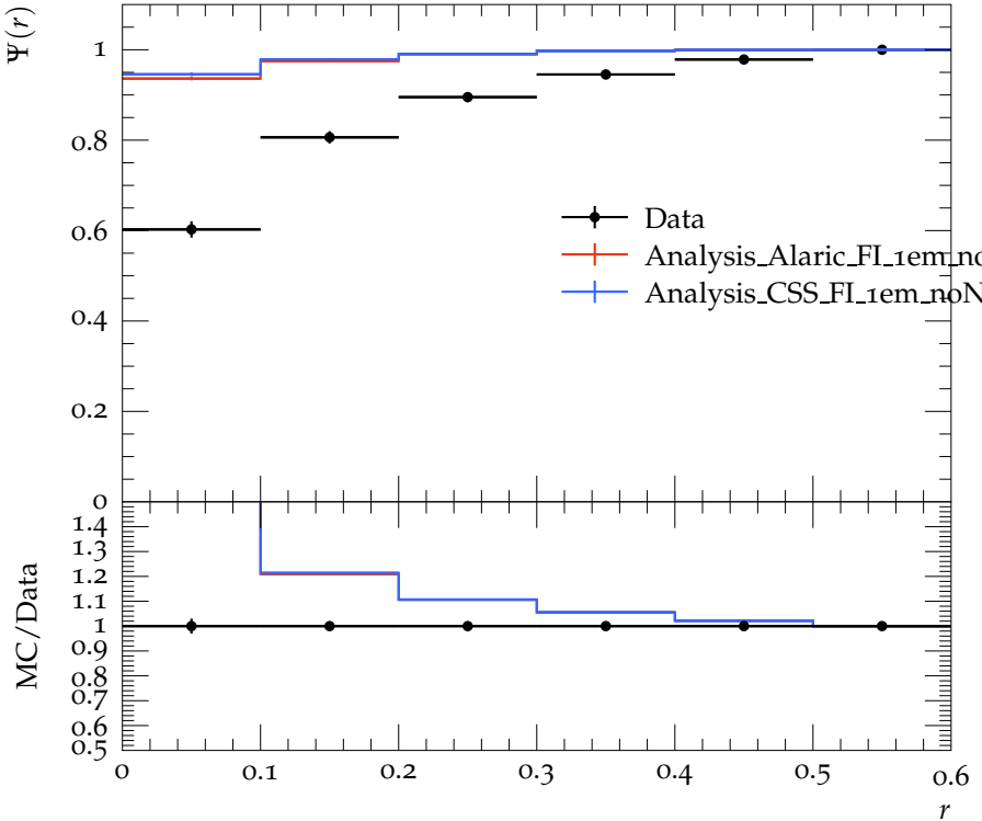
Jet shape \Psi for p_{\perp} \in 80\text{--}110\text{ GeV} , y \in 2.1\text{--}2.8
