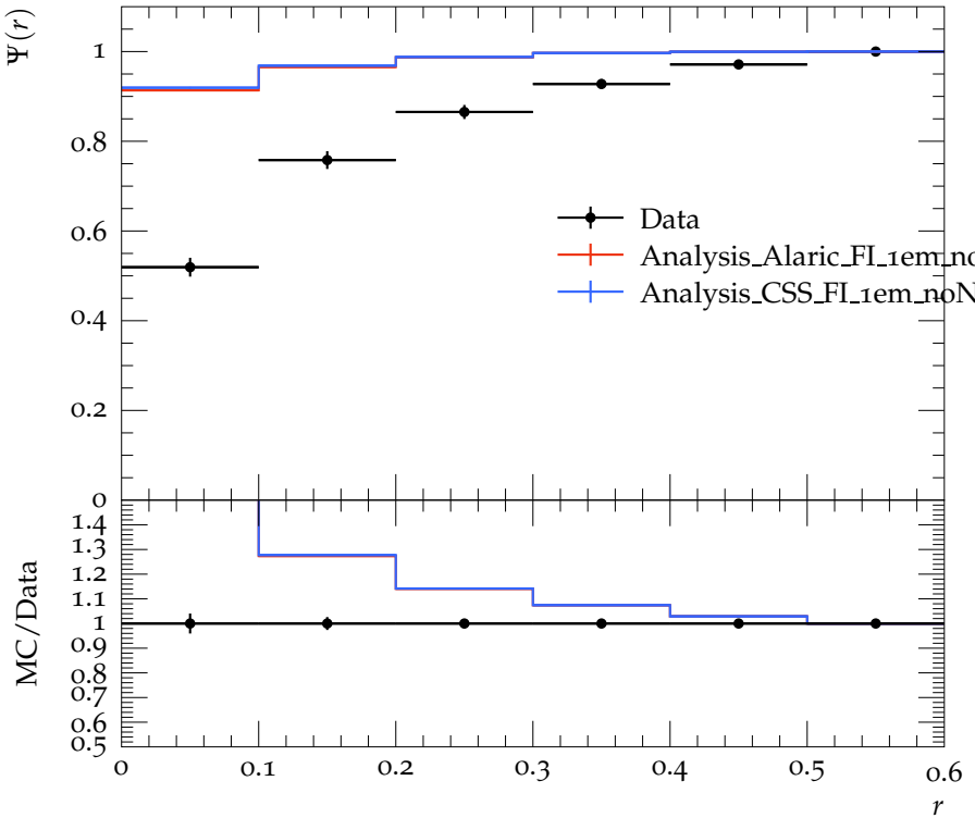
Jet shape \Psi for p_{\perp} \in 60\text{--}80\text{ GeV} , y \in 0.0\text{--}2.8
