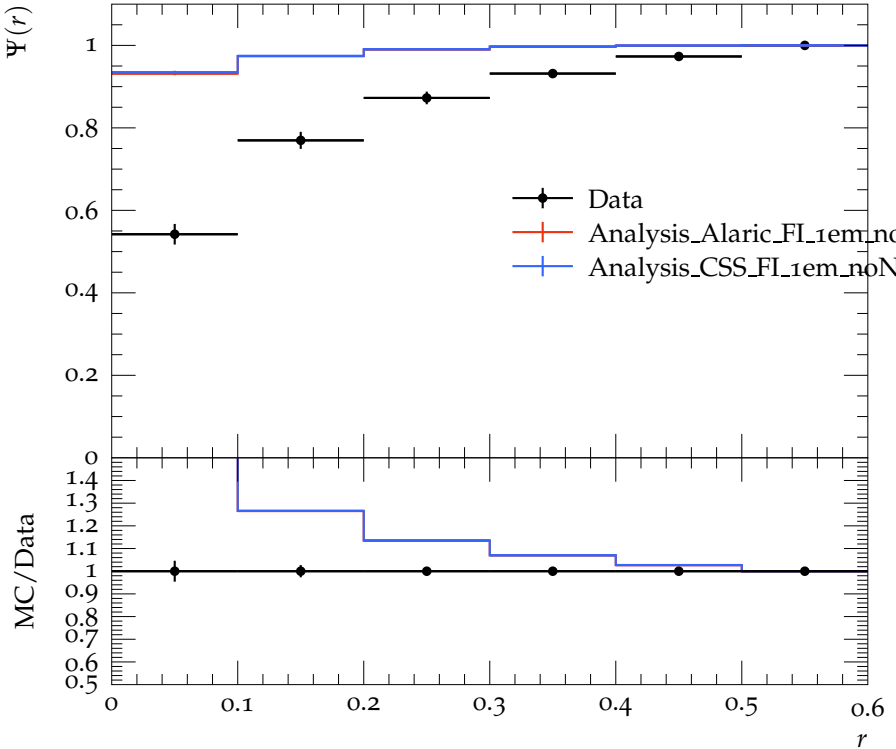
Jet shape \Psi for p_{\perp} \in 60\text{--}80\text{ GeV} , y \in 2.1\text{--}2.8
