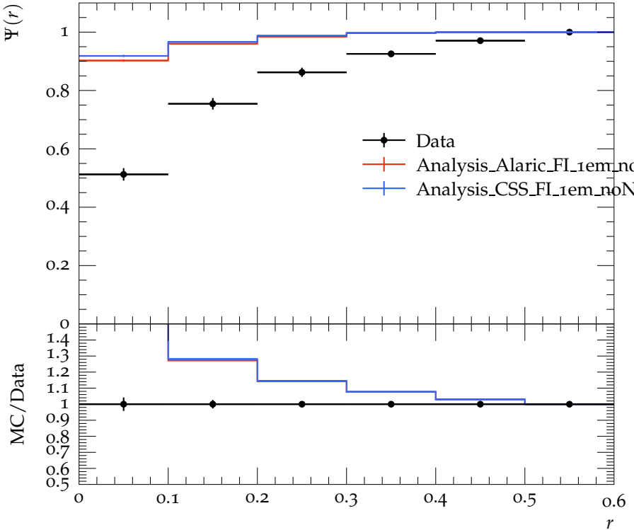
Jet shape \Psi for p_{\perp} \in 60\text{--}80\text{ GeV} , y \in 0.3\text{--}0.8
