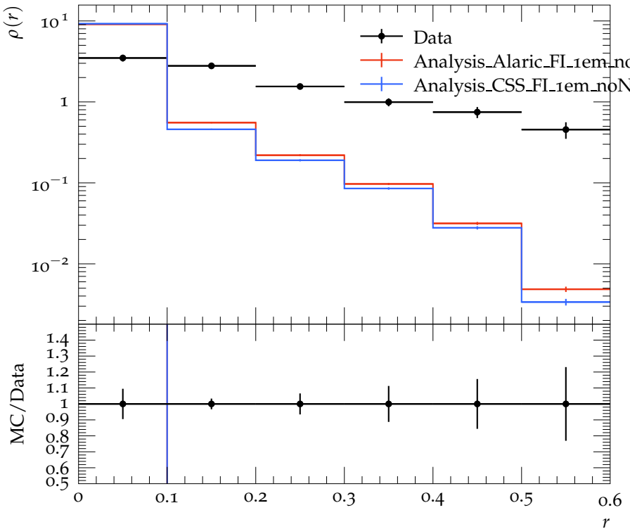
Jet shape \rho for p_{\perp} \in 30\text{--}40\text{ GeV} , y \in 0.0\text{--}2.8
