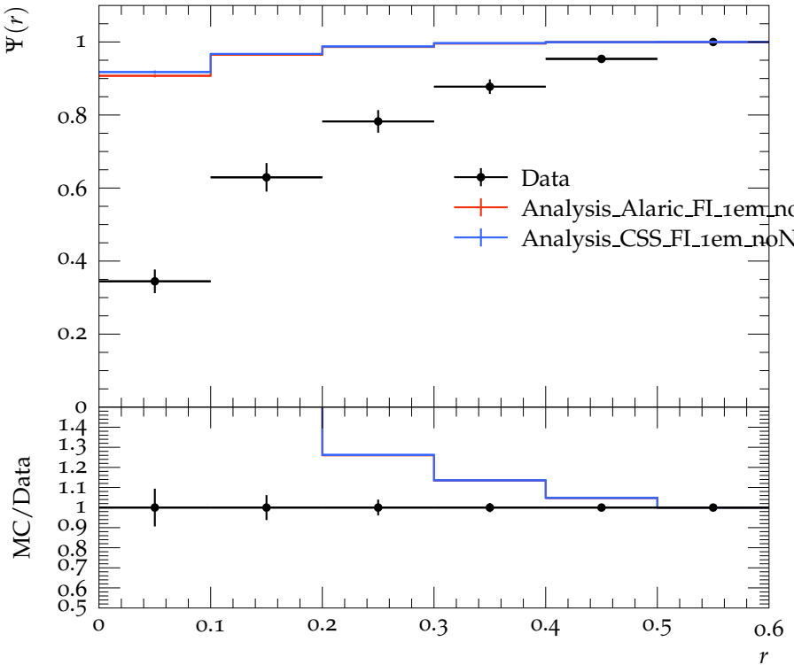
Jet shape \Psi for p_{\perp} \in 30\text{--}40\text{ GeV} , y \in 0.0\text{--}0.3
