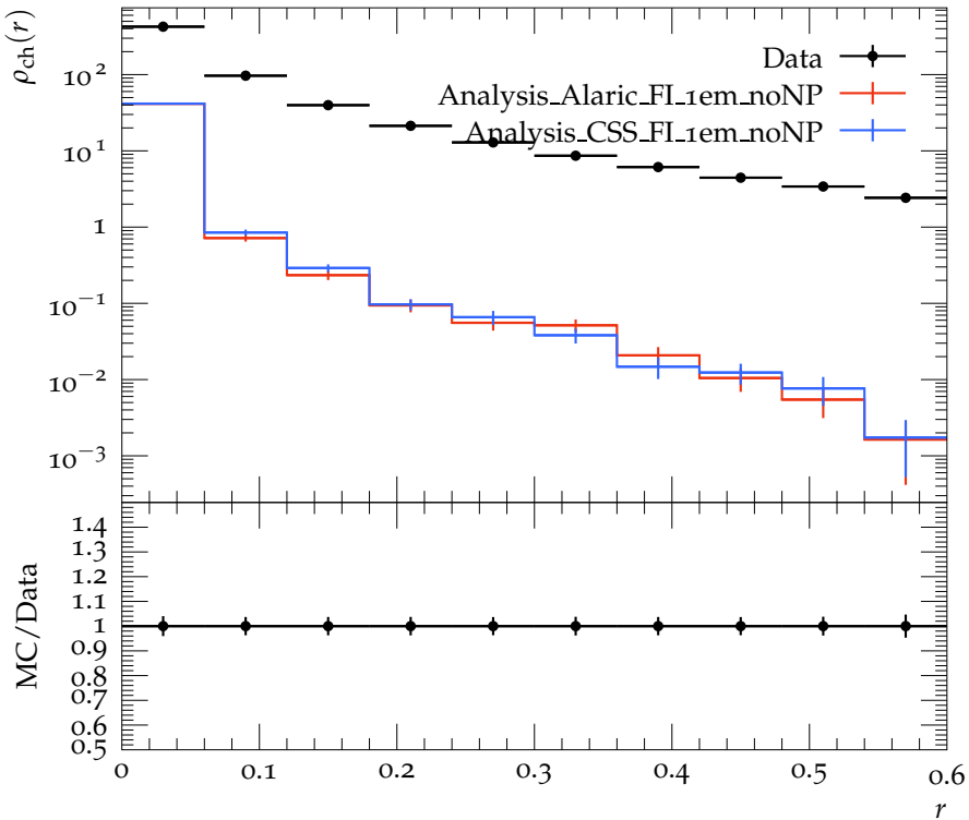
Density of charged particles for 310 \text{ GeV} < p_{T \text{ jet}} < 400 \text{ GeV}
