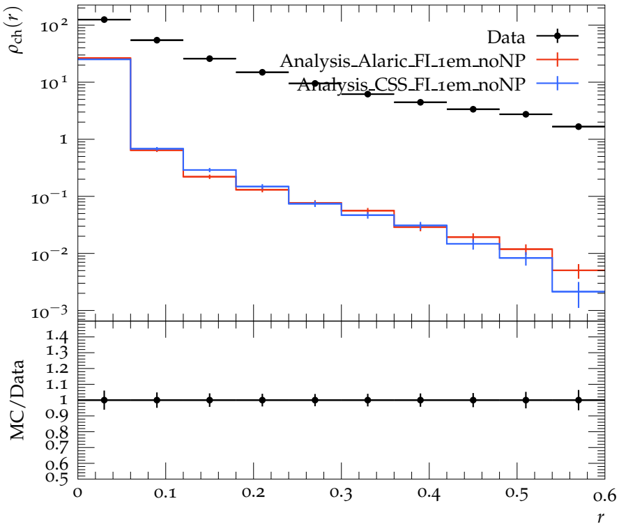
Density of charged particles for 60 \text{ GeV} < p_{T \text{ jet}} < 80 \text{ GeV}
