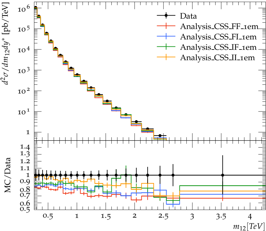
Dijet double-differential cross sections ( y^* < 0.5 ), R=0.6
