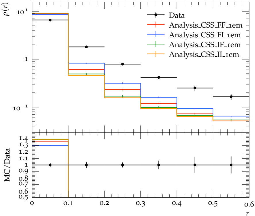
Jet shape \rho for p_{\perp} \in 160\text{--}210 GeV, y \in 0.0\text{--}0.3
