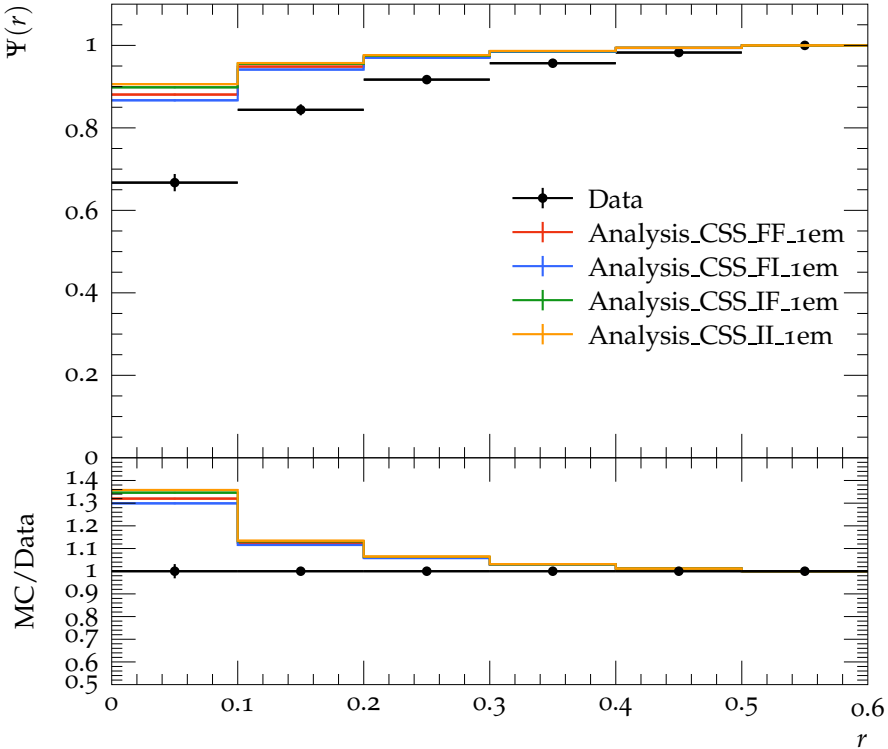
Jet shape \Psi for p_{\perp} \in 110\text{--}160\text{ GeV} , y \in 2.1\text{--}2.8
