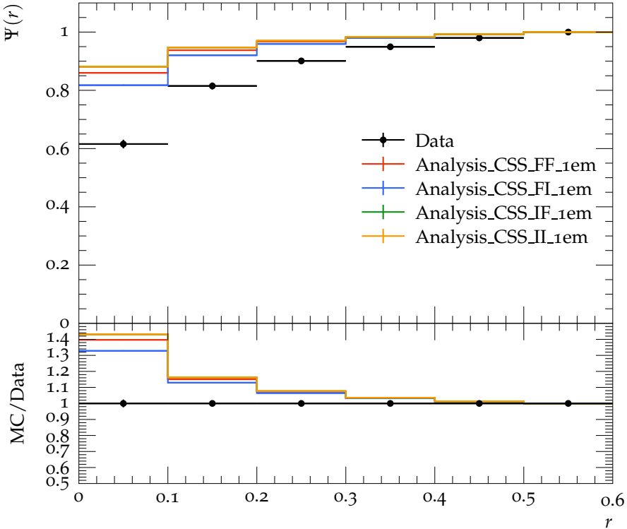
Jet shape \Psi for p_{\perp} \in 110\text{--}160\text{ GeV} , y \in 0.0\text{--}0.3
