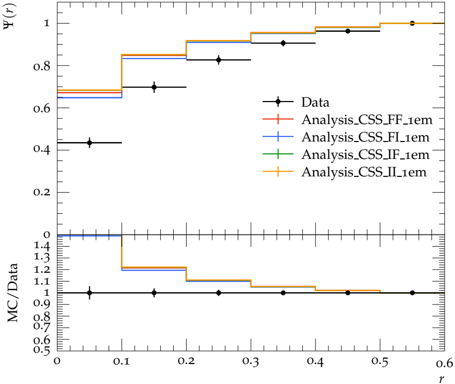
Jet shape \Psi for p_{\perp} \in 40\text{--}60\text{ GeV} , y \in 0.0\text{--}2.8
