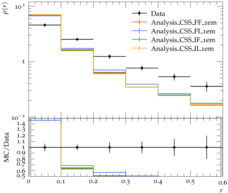
Jet shape \rho for p_{\perp} \in 40\text{--}60\text{ GeV} , y \in 2.1\text{--}2.8
