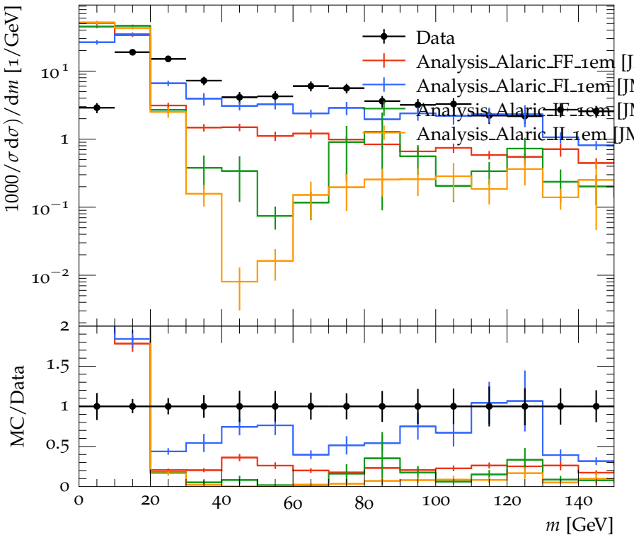
Pruned AK7 dijets, (p_T^1 + p_T^2)/2 = 1000\text{--}1500 GeV
