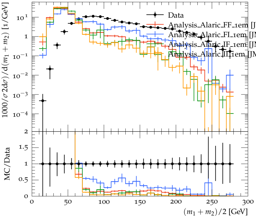
Filtered AK7 dijets, (p_T^1 + p_T^2)/2 = 1000\text{--}1500 GeV
