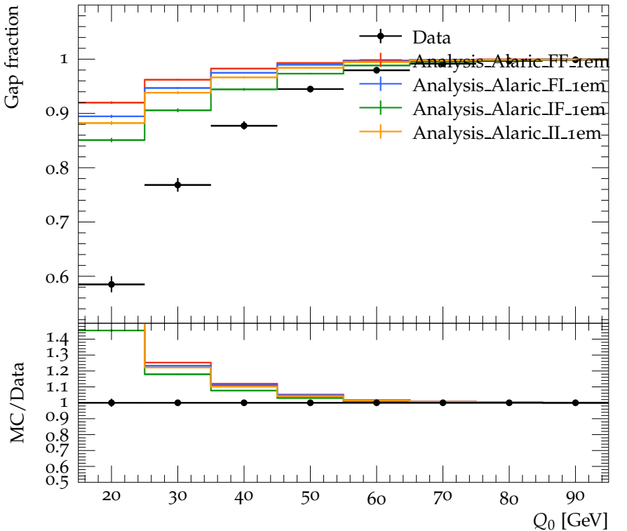
Gap fraction as a function of Q_0 for events satisfying 3 < \Delta y \leq 4
