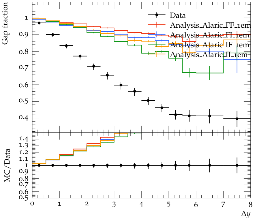
Gap fraction as a function of leading dijet rapidity separation
