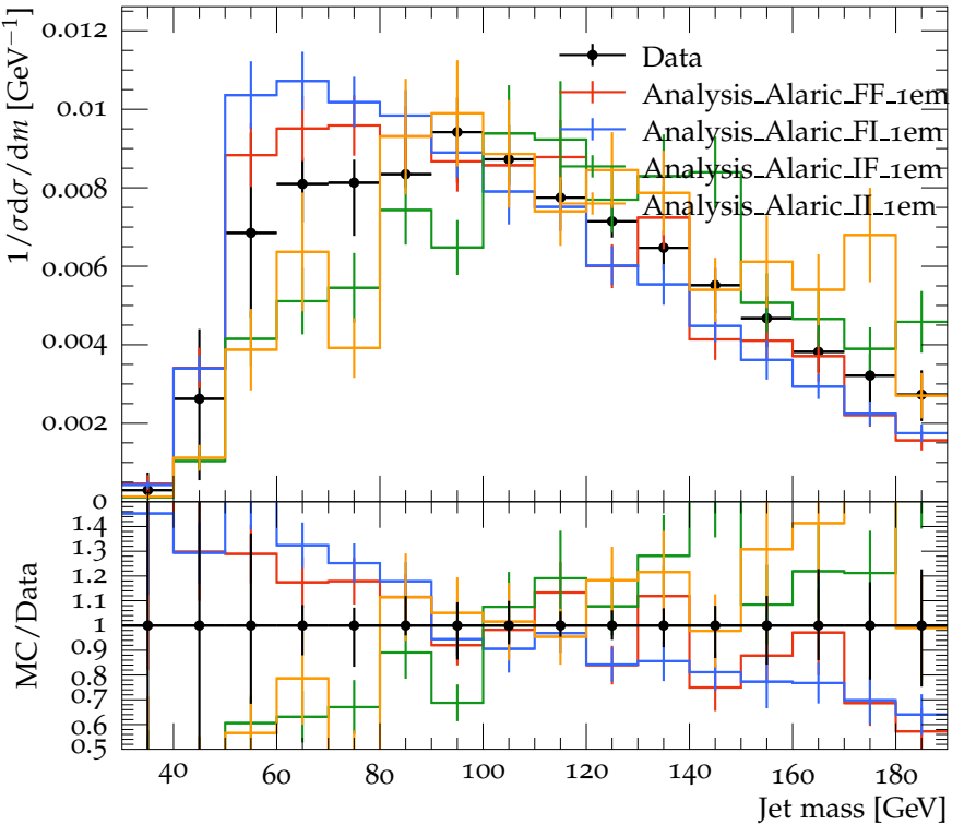
Cambridge-Aachen filtered jets, R=1.2 , 300 \text{ GeV} < p_{\perp} < 400 \text{ GeV}
