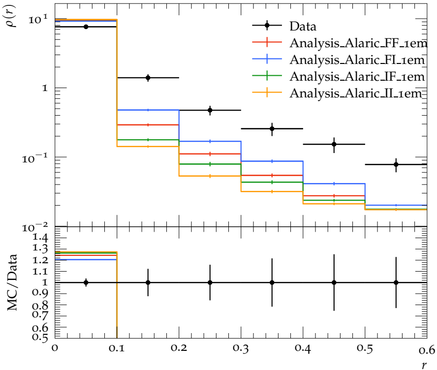
Jet shape \rho for p_{\perp} \in 500\text{--}600 GeV, y \in 0.0\text{--}2.8
