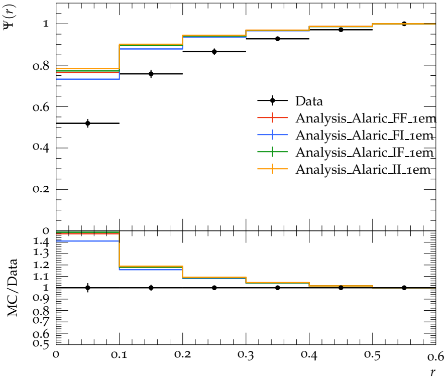
Jet shape \Psi for p_{\perp} \in 60\text{--}80\text{ GeV} , y \in 0.0\text{--}2.8
