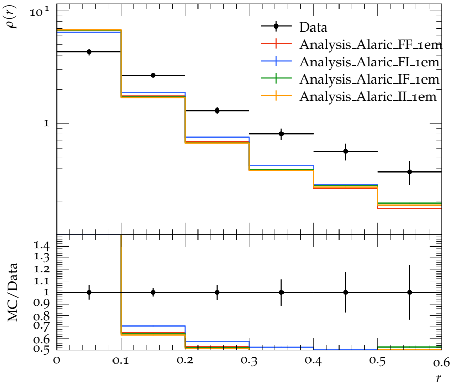
Jet shape \rho for p_{\perp} \in 40\text{--}60\text{ GeV} , y \in 1.2\text{--}2.1
