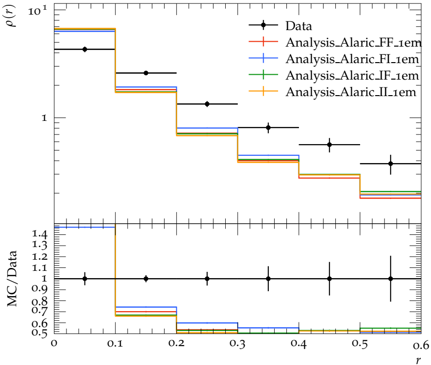
Jet shape \rho for p_{\perp} \in 40\text{--}60\text{ GeV} , y \in 0.0\text{--}0.3
