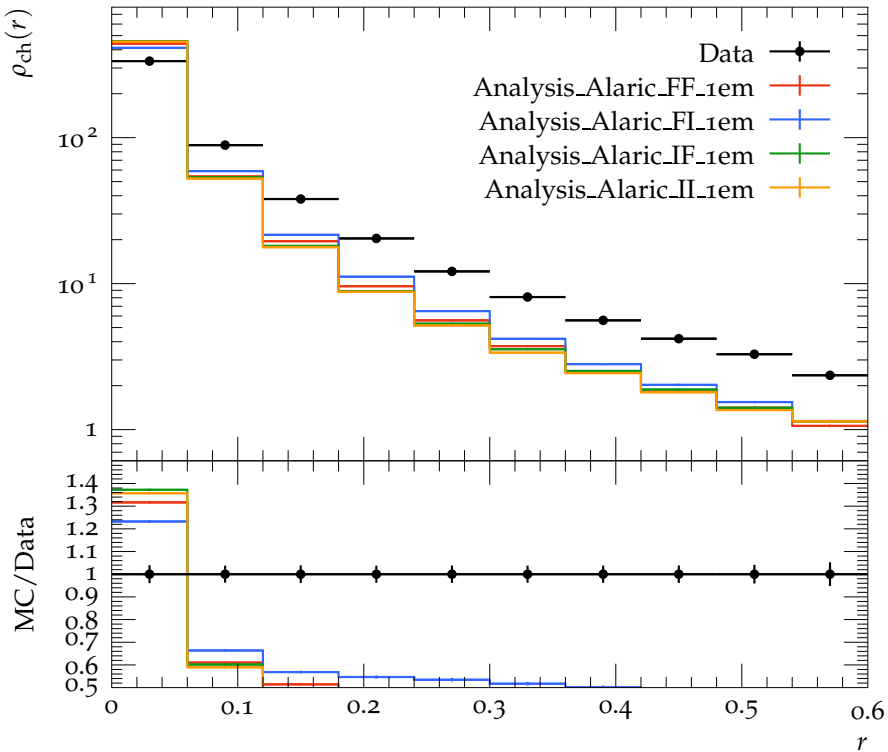
Density of charged particles for 210 \text{ GeV} < p_{T \text{ jet}} < 260 \text{ GeV}
