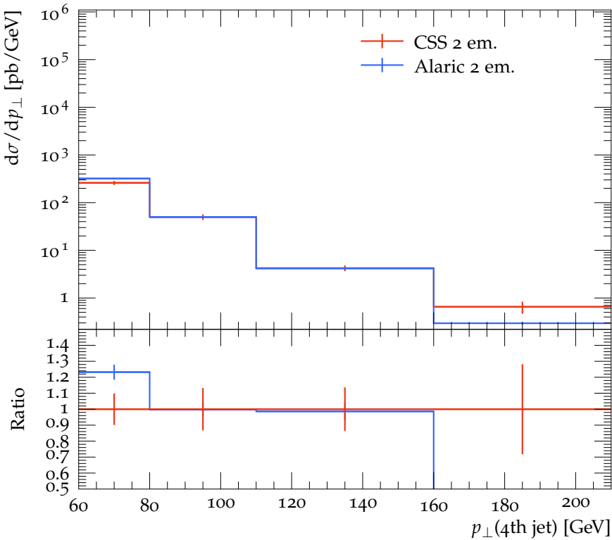
Transverse momentum of the 4th leading jet ( R = 0.4 )
