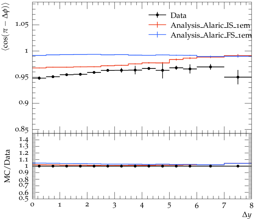
\langle \cos(\pi - \Delta\phi) \rangle for gap events as a function of \Delta y
