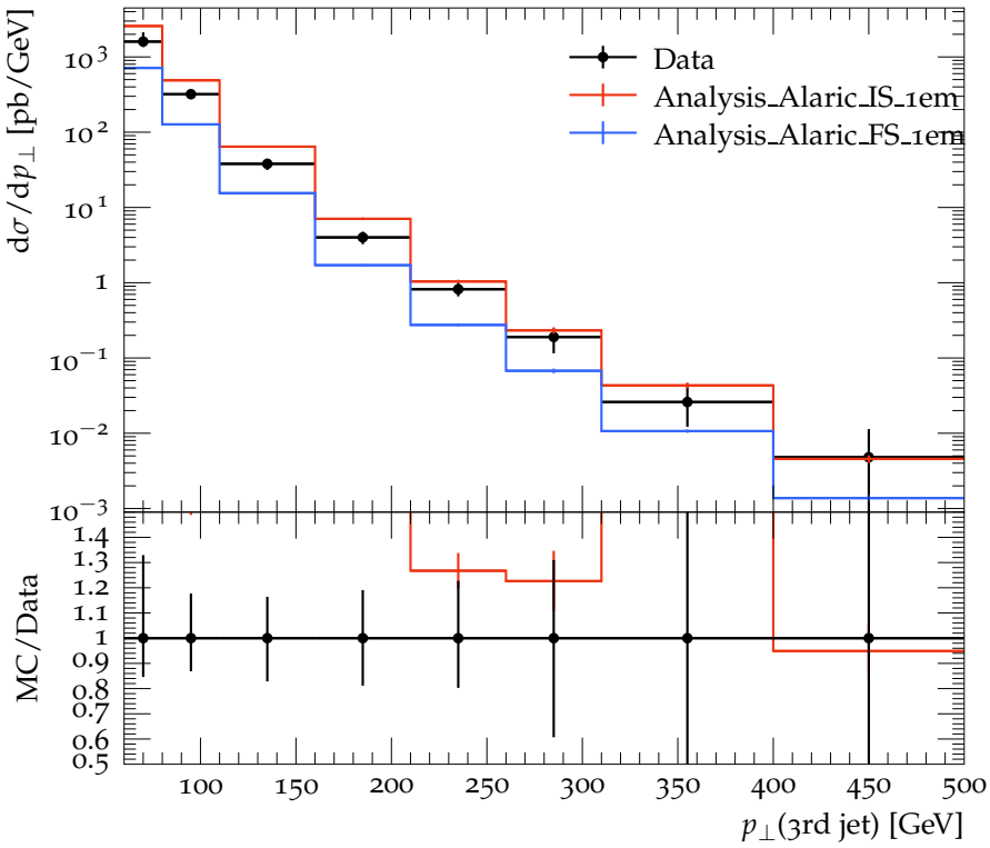
Transverse momentum of the 3rd leading jet ( R = 0.4 )
