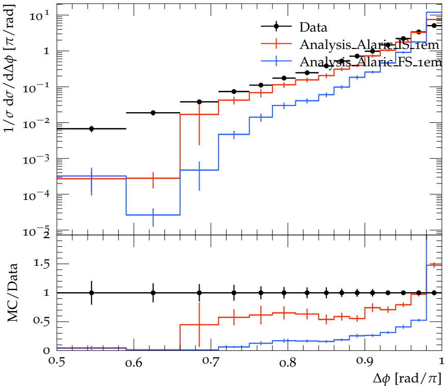
Dijet azimuthal decorrelations for 110 < p_{\perp}^{\max}/\text{GeV} < 160
