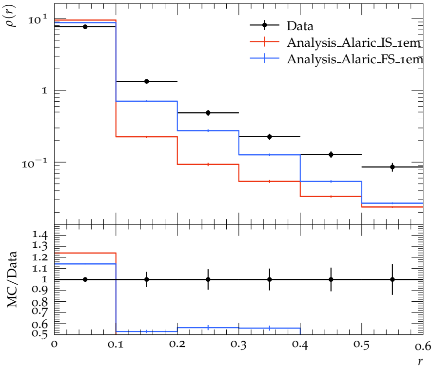
Jet shape \rho for p_{\perp} \in 400\text{--}500 GeV, y \in 0.0\text{--}2.8
