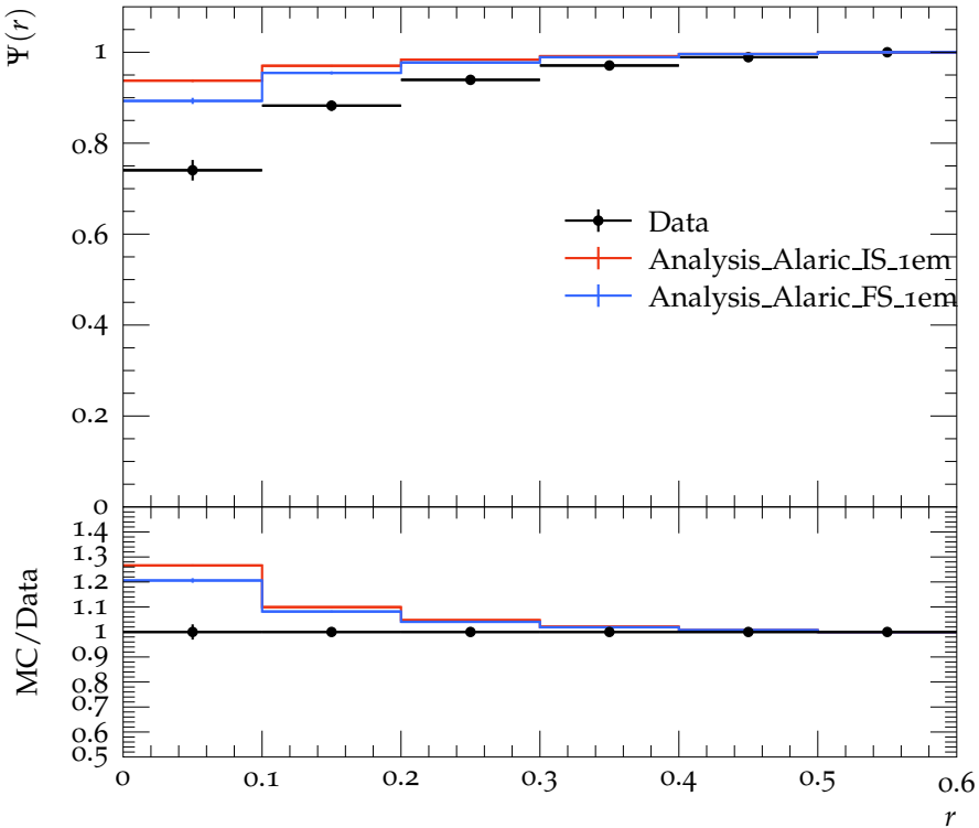
Jet shape \Psi for p_{\perp} \in 210\text{--}260 GeV, y \in 2.1\text{--}2.8
