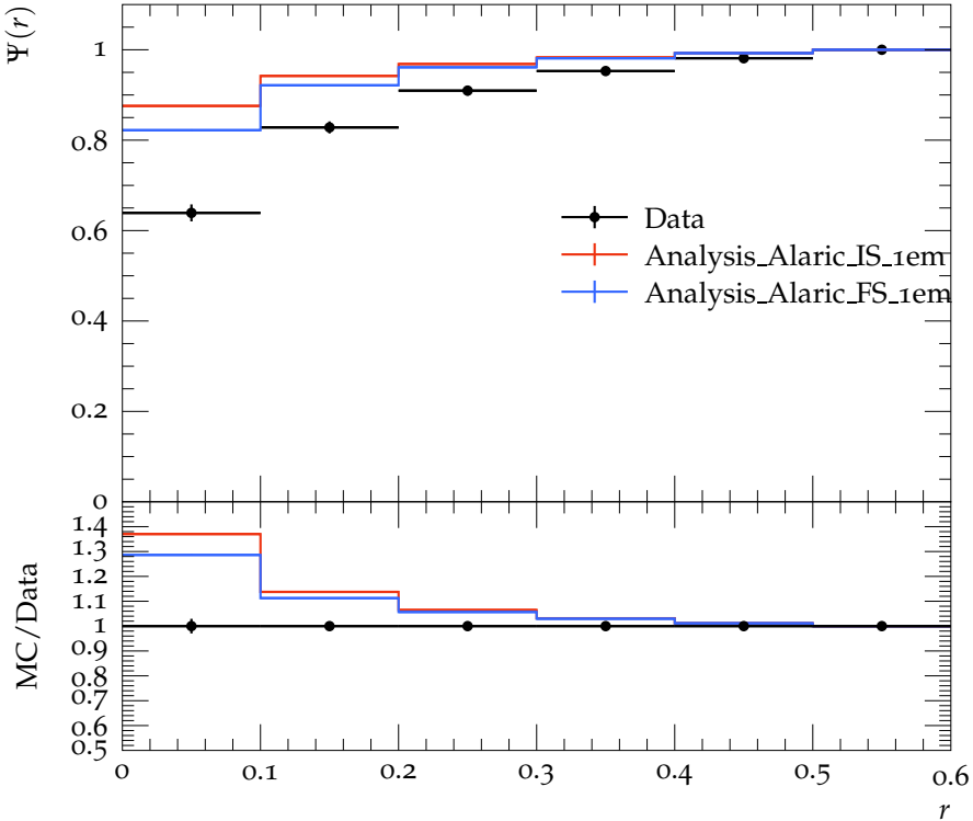
Jet shape \Psi for p_{\perp} \in 110\text{--}160\text{ GeV} , y \in 1.2\text{--}2.1
