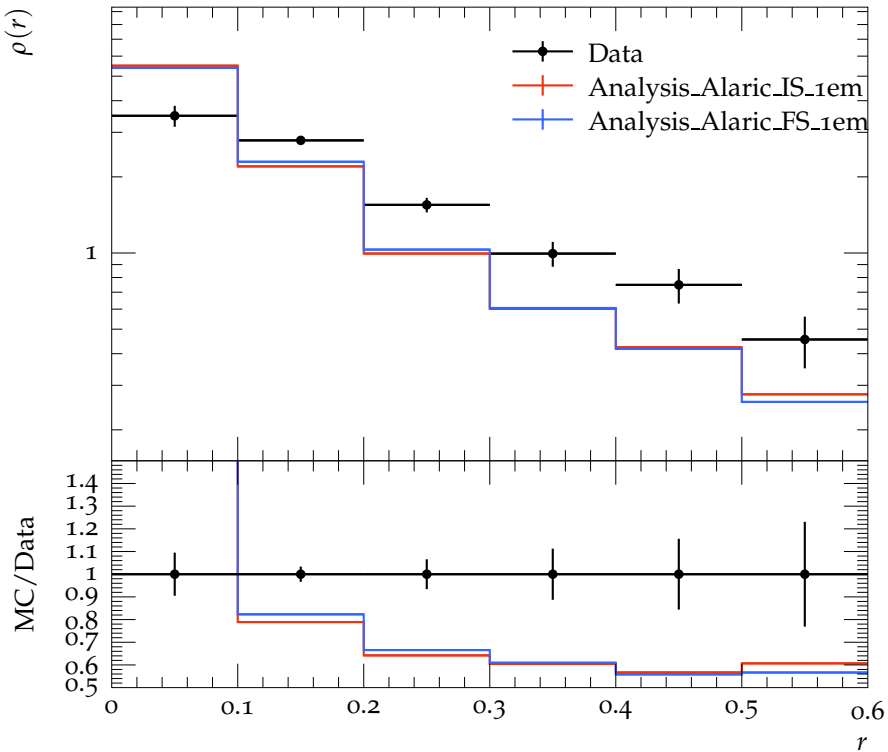
Jet shape \rho for p_{\perp} \in 30\text{--}40\text{ GeV} , y \in 0.0\text{--}2.8
