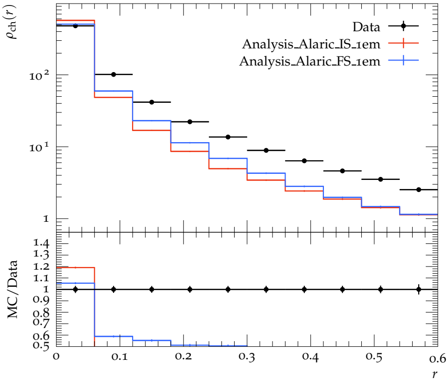
Density of charged particles for 400 \text{ GeV} < p_{T \text{ jet}} < 500 \text{ GeV}
