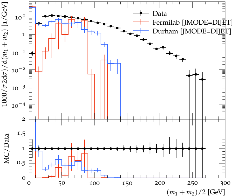
Trimmed AK7 dijets, (p_T^1 + p_T^2)/2 = 600\text{--}800 GeV
