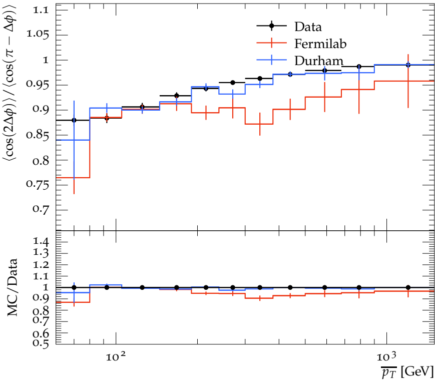
\langle \cos(2\Delta\phi) \rangle / \langle \cos(\pi - \Delta\phi) \rangle for gap events as a function of \overline{p_T}
