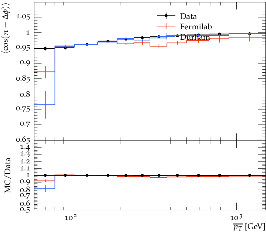
\langle \cos(\pi - \Delta\phi) \rangle for gap events as a function of \overline{p_T}
