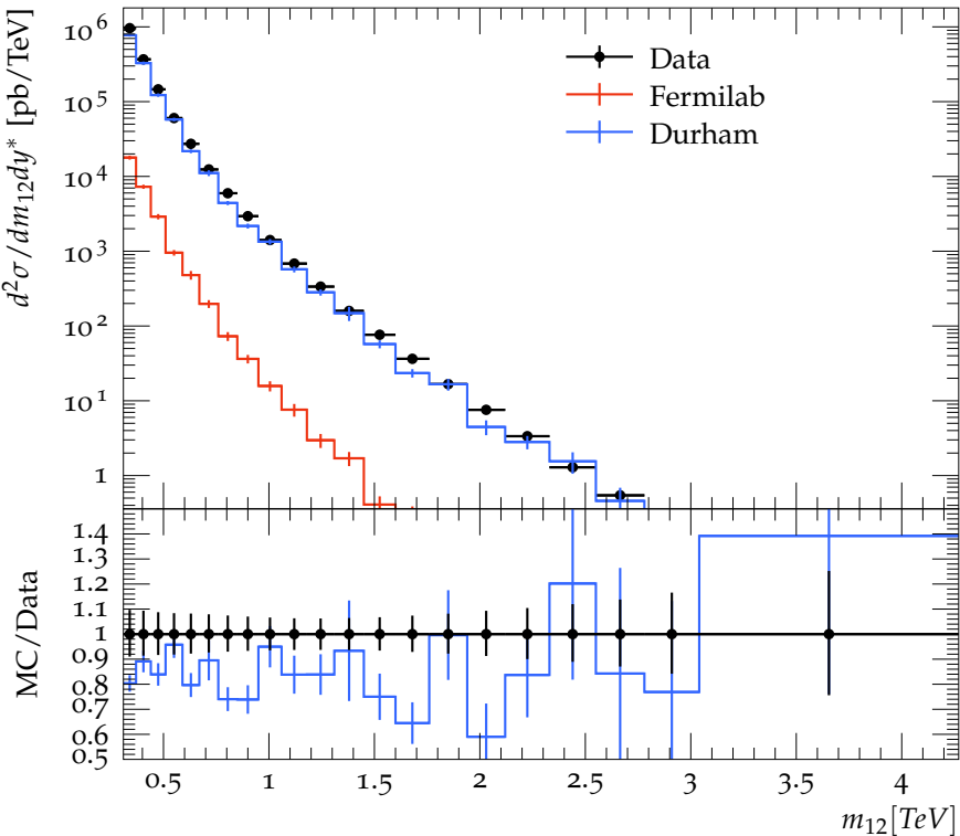
Dijet double-differential cross sections ( 0.5 < y^* < 1.0 ), R=0.6
