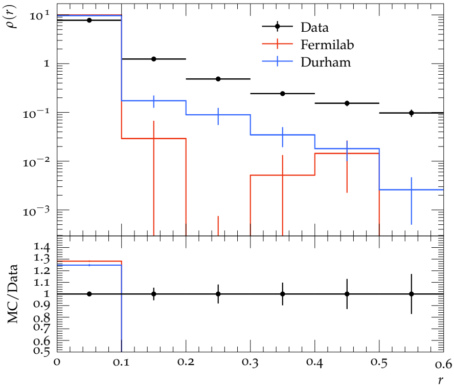
Jet shape \rho for p_{\perp} \in 310\text{--}400 GeV, y \in 1.2\text{--}2.1
