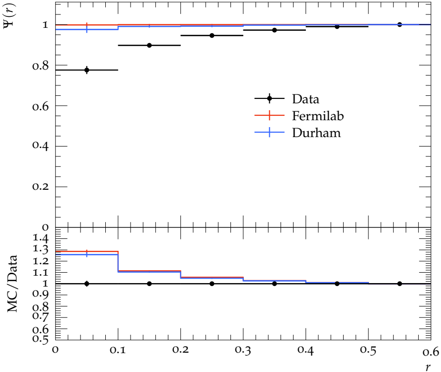
Jet shape \Psi for p_{\perp} \in 260\text{--}310\text{ GeV} , y \in 2.1\text{--}2.8
